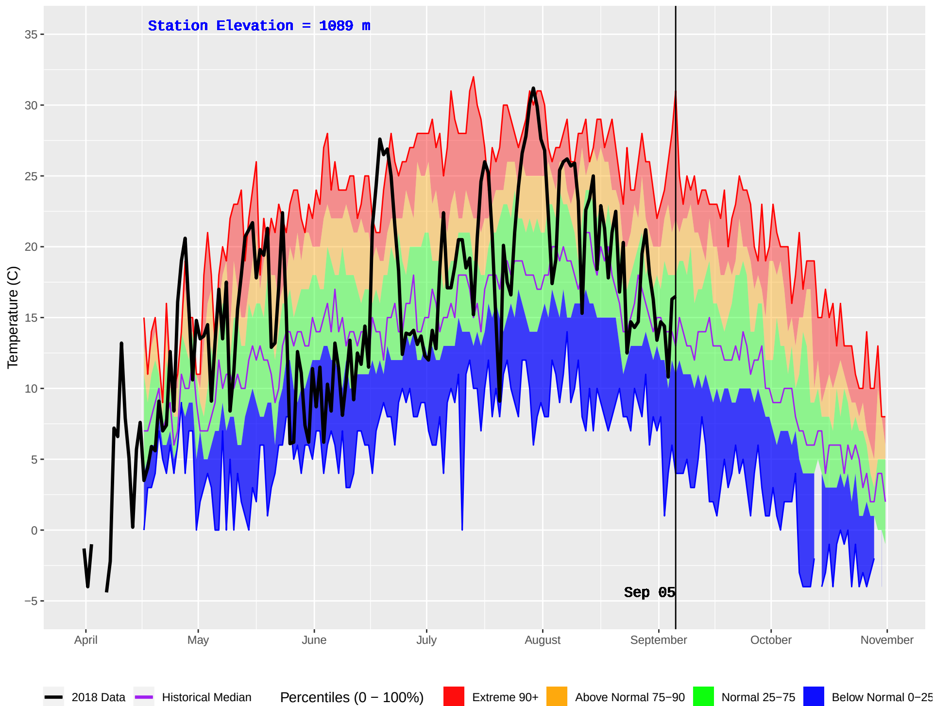
EAST OOTSA (170) : Historical (1986–2016) and Current (2018) Daily Temperature
