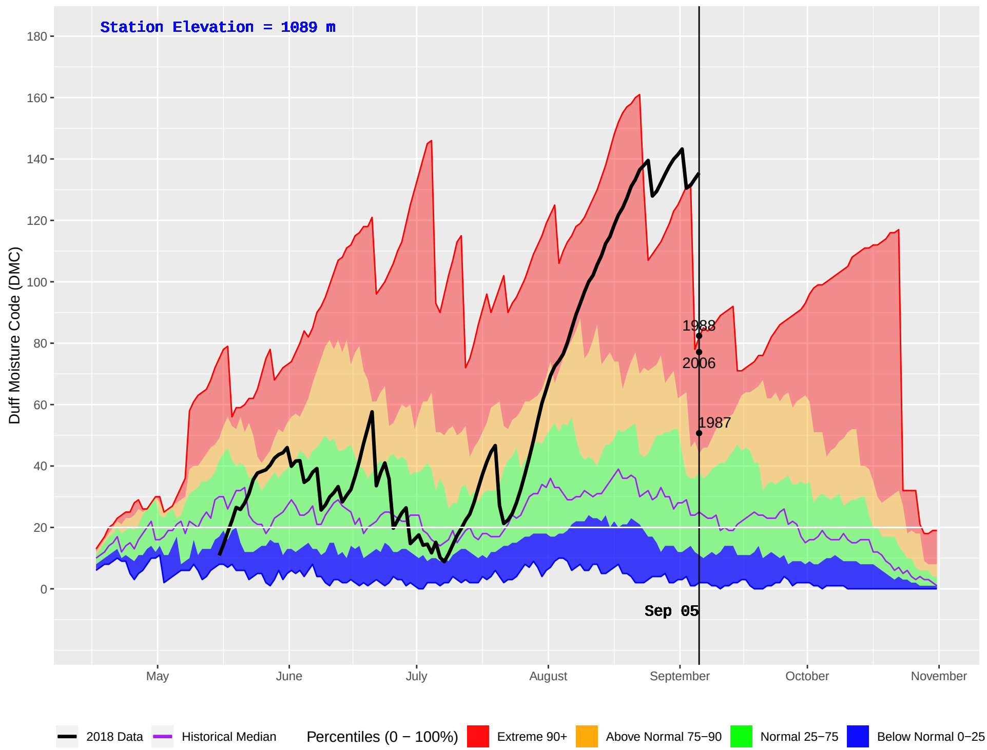
EAST OOTSA (170) : Historical (1986–2016) and Current (2018) Daily Duff Moisture Code (DMC)
